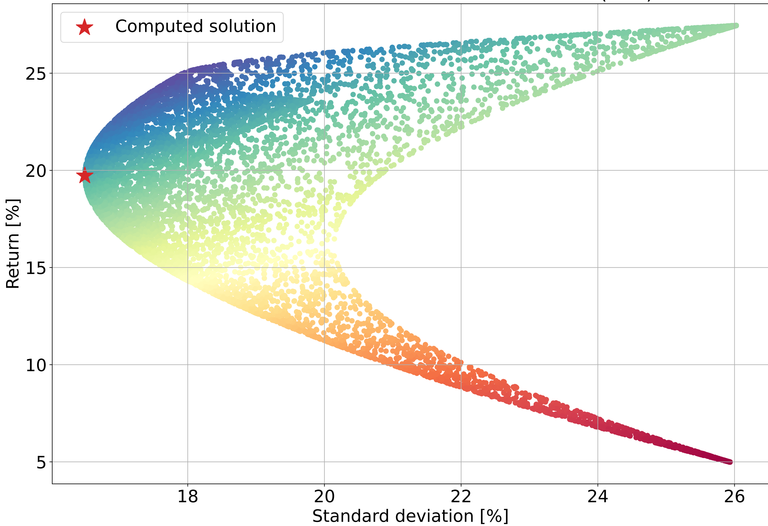
Montecarlo on Ytrain -- Markovitz Probabilistic (n=3)
